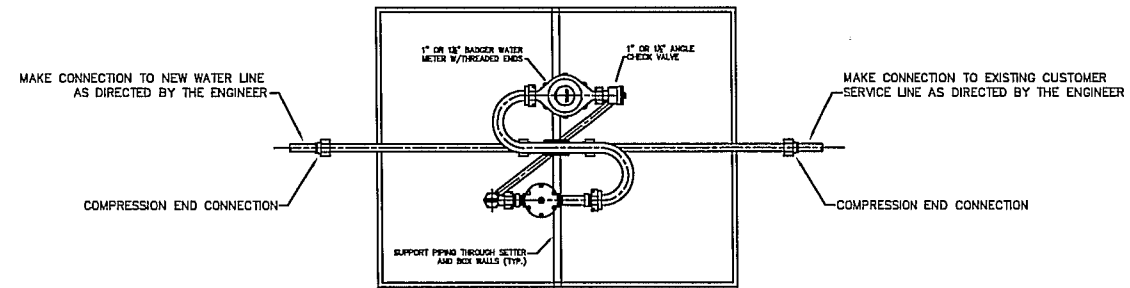
1" AND 1-1/2" METER VAULT PLAN
