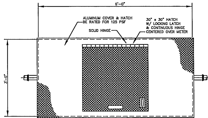
2" AND 3" METER VAULT COVER/HATCH PLAN
