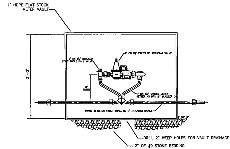
1" AND 1-1/2" METER VAULT SECTION
