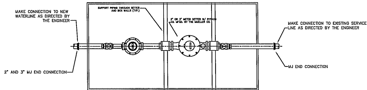
2" AND 3" METER VAULT PLAN
