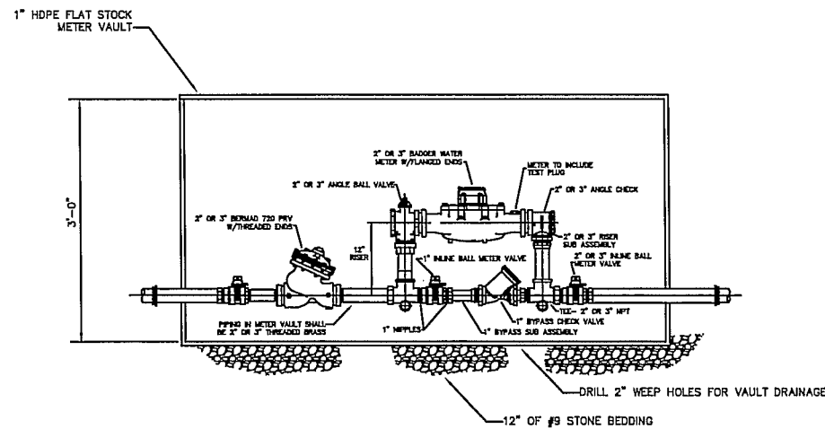
2" AND 3" METER VAULT SECTION
