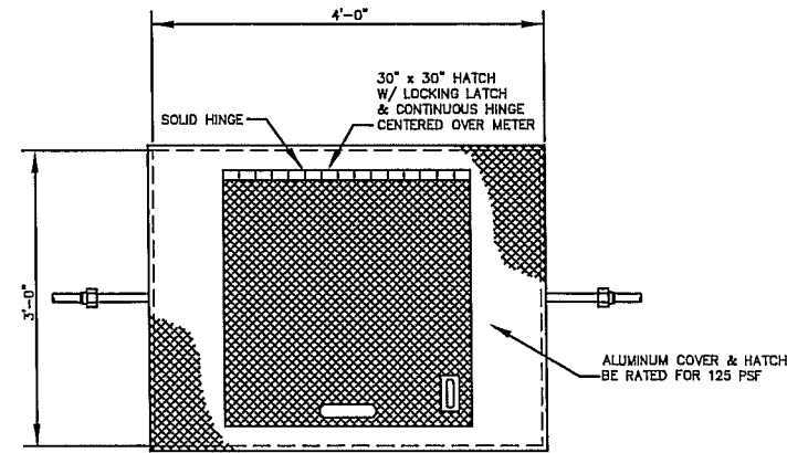
1" AND 1-1/2" METER VAULT COVER/HATCH PLAN
