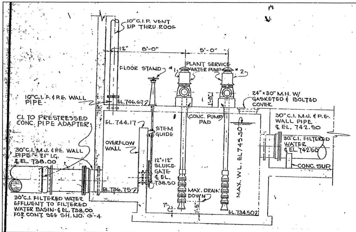
EXHIBIT 5-37 Pit Layout
