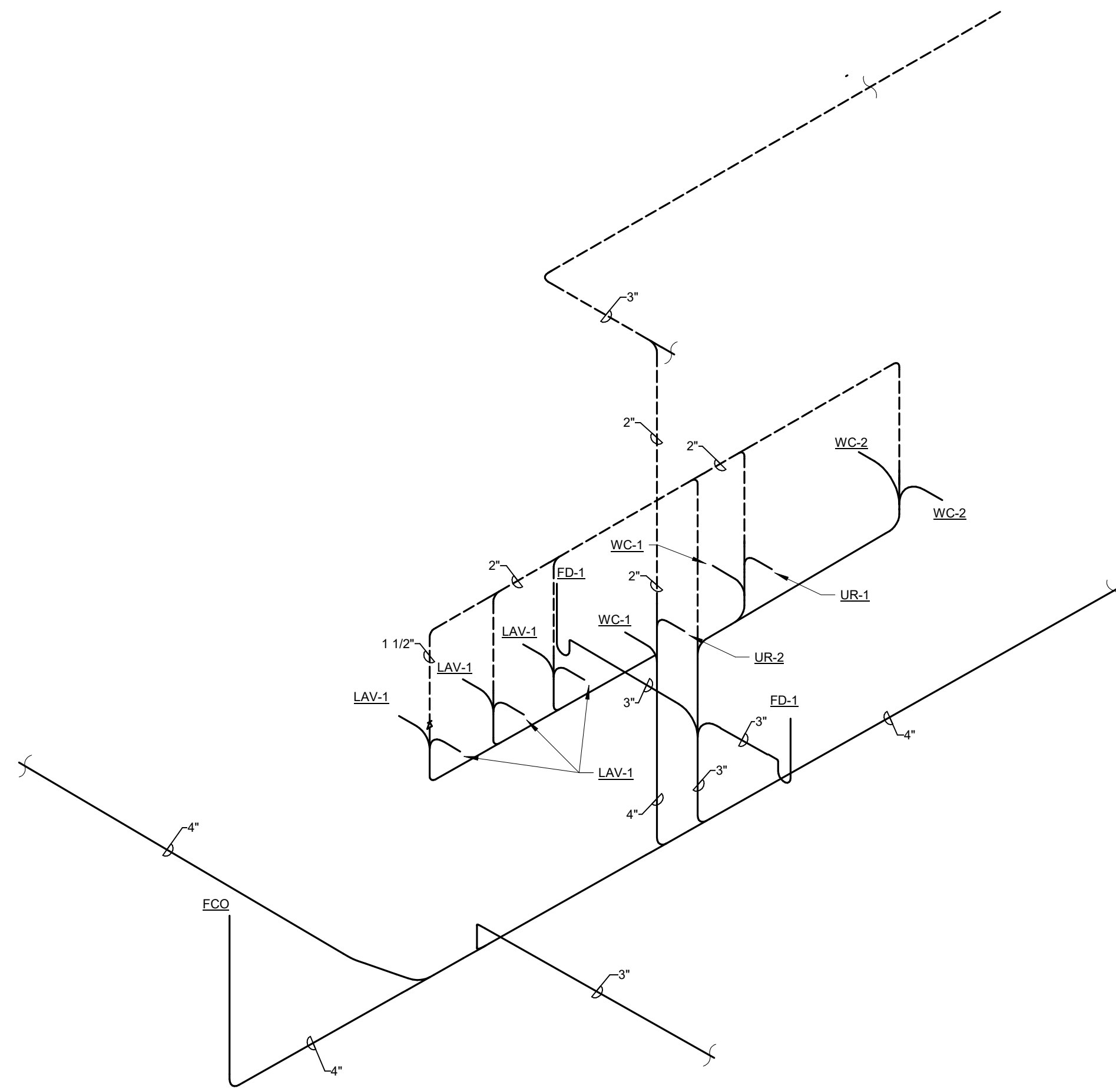
6 PLUMBING WASTE & VENT ISOMETRIC PLAN - OFFICE ROOMS 155 & 156 NOT TO SCALE
