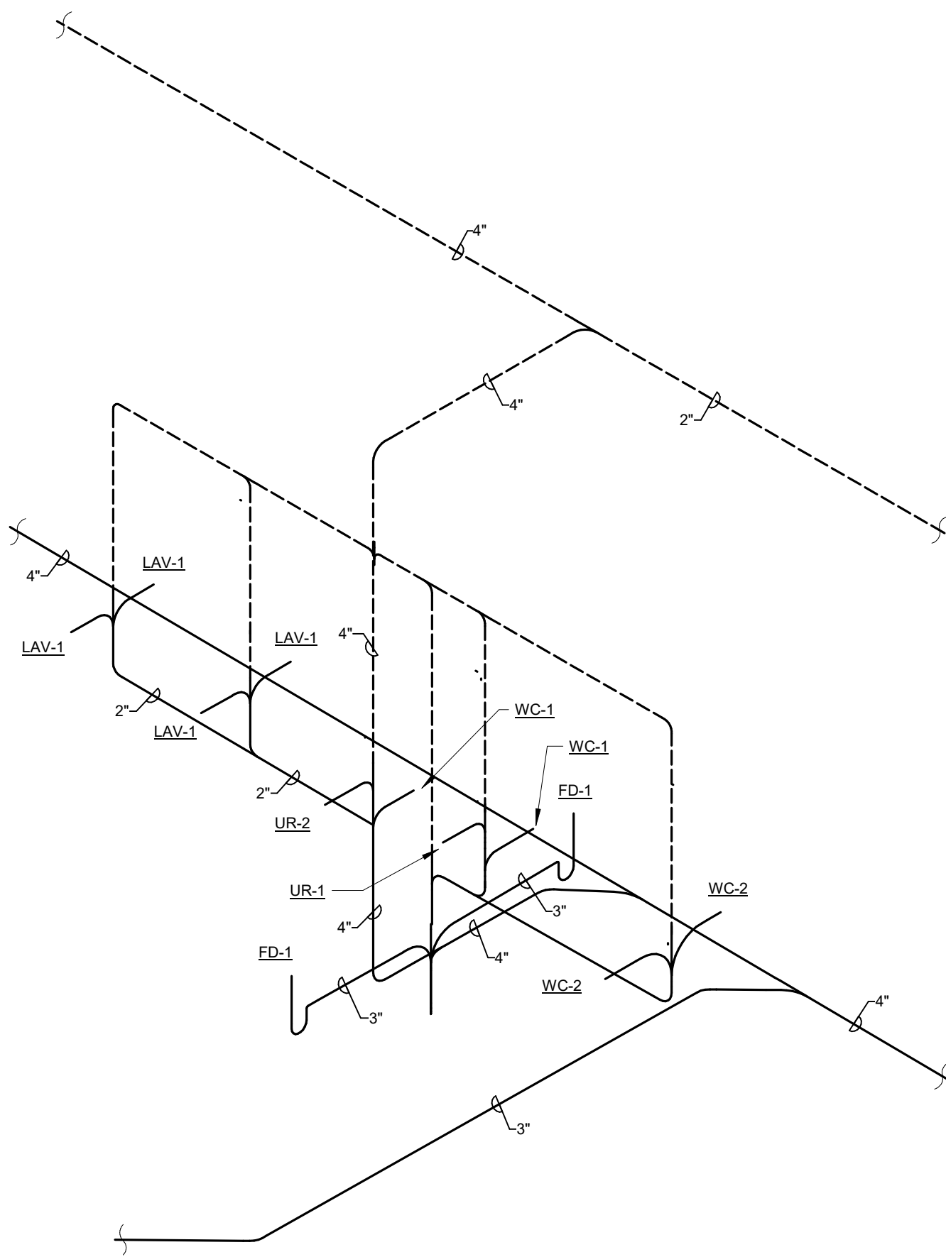
5 PLUMBING WASTE & VENT ISOMETRIC PLAN - OFFICE ROOMS 122 & 123 NOT TO SCALE
