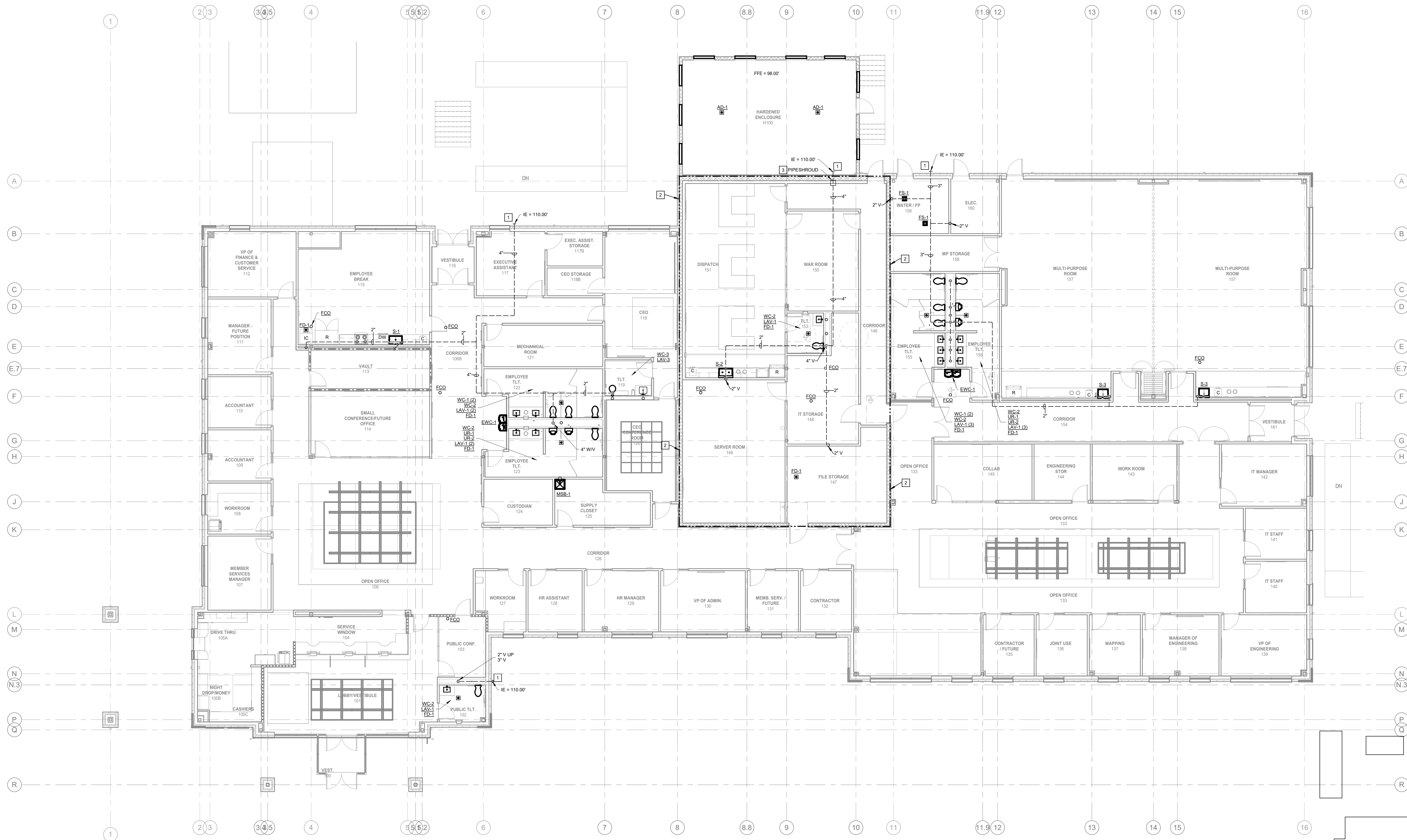
FIRST FLOOR PLUMBING WASTE AND VENT PLAN - OFFICE SCALE: 1/8" = 1'-0" NORTH F.F.E. = 100.00' (CIVIL = 895.30')
