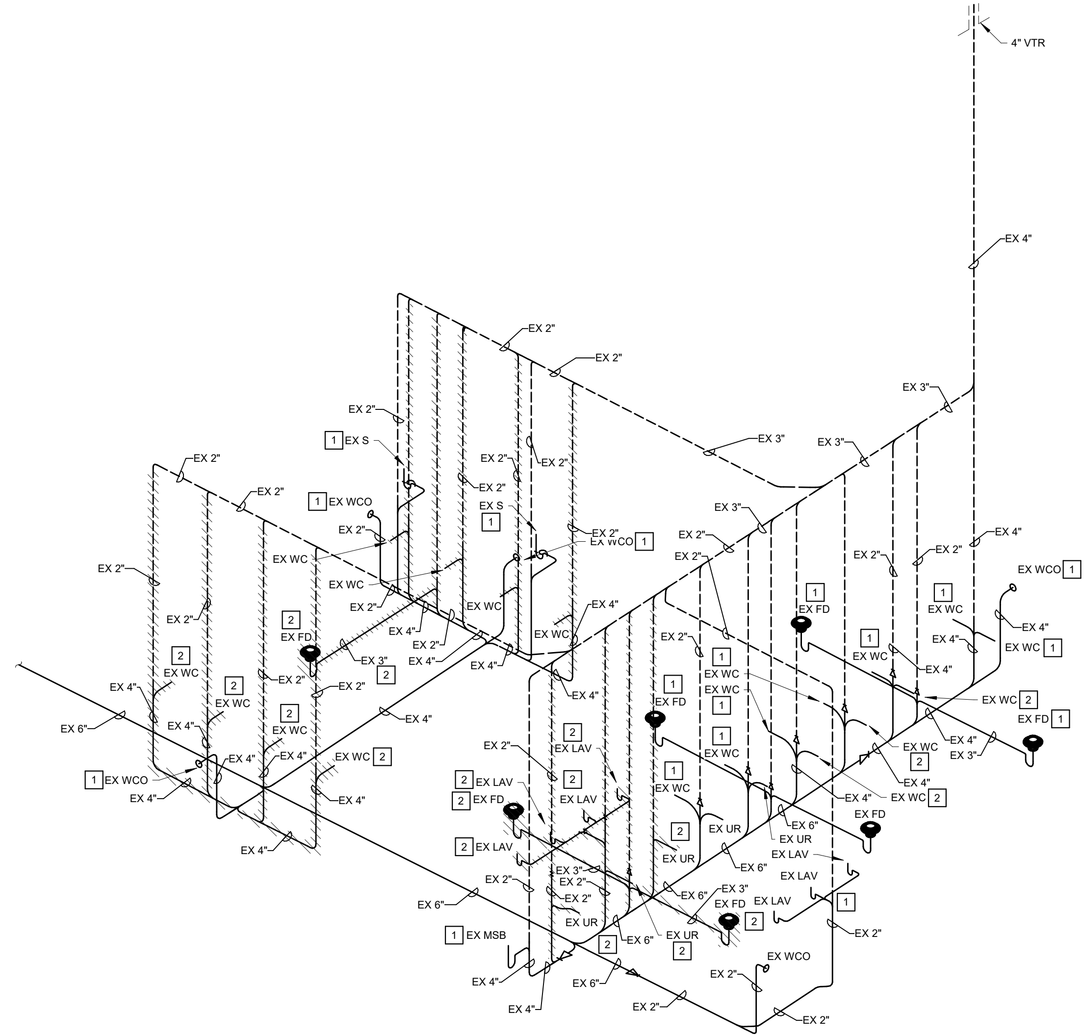
PLUMBING WASTE & VENT ISOMETRIC PLAN - EXISTING NOT TO SCALE
