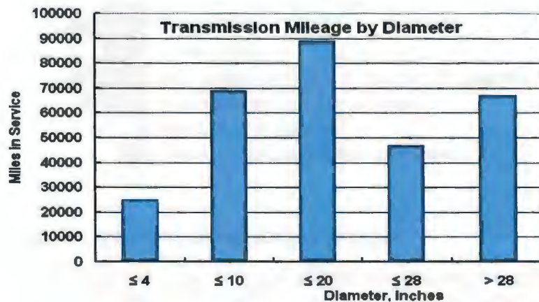
Figure 2. Mileage of transmission pipelines by diameter
