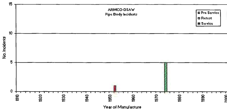
Figure F2. ARMCO DSAW pipe body incidents by year
