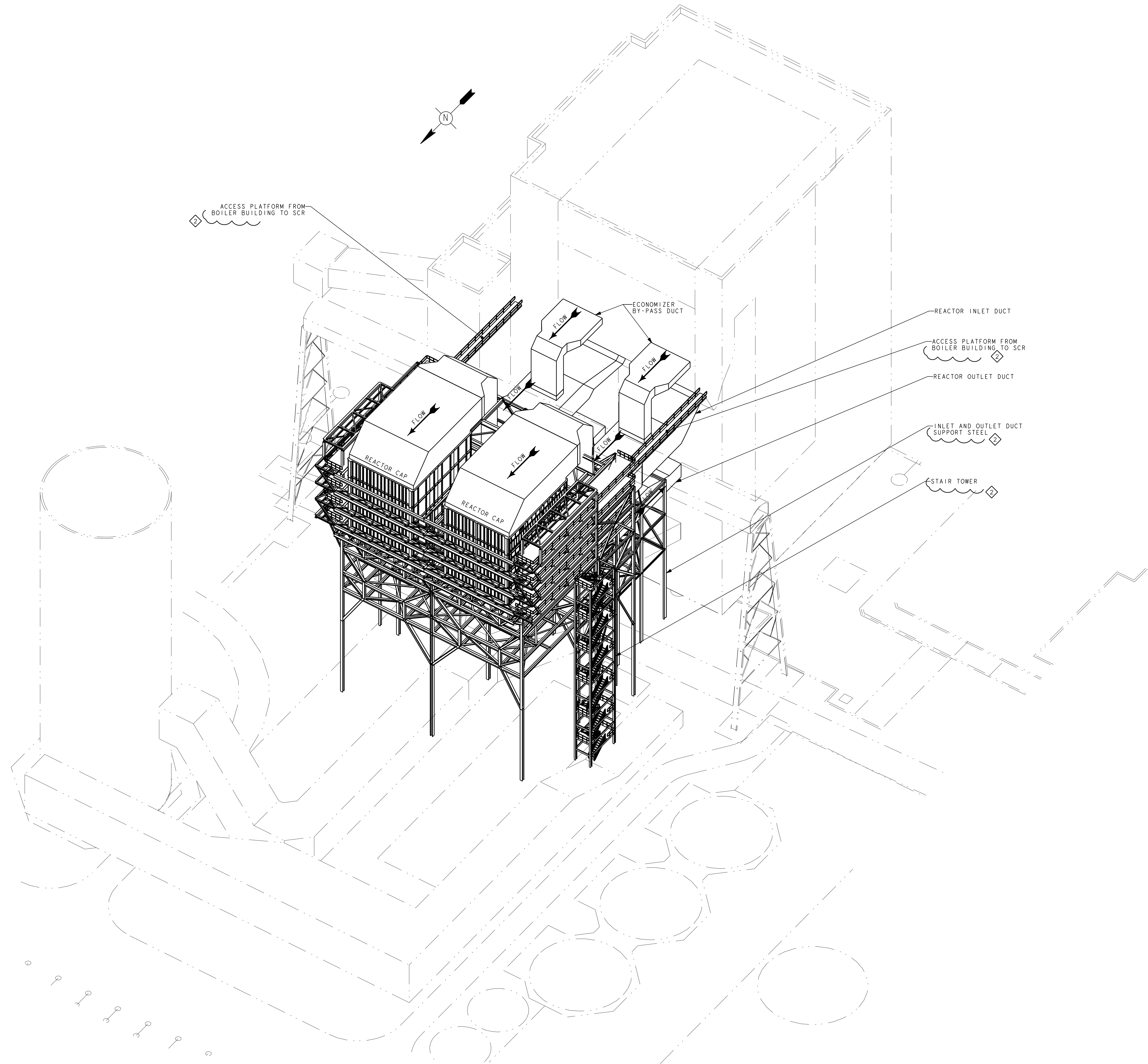
ISOMETRIC VIEW (LOOKING SOUTHEAST)
