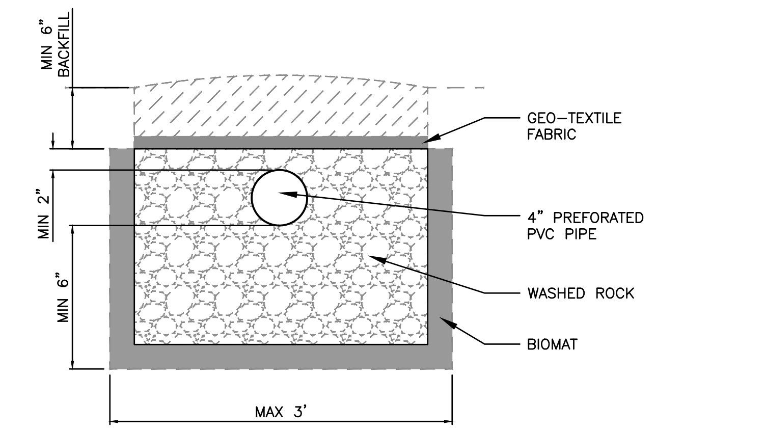
PERFORATED PIPE DETAIL
