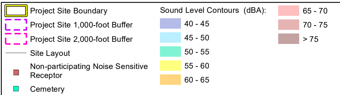
Figure 2 Received Sound Levels, Pile Driving Activities Bluegrass Plains Solar Project Fayette County, Kentucky
