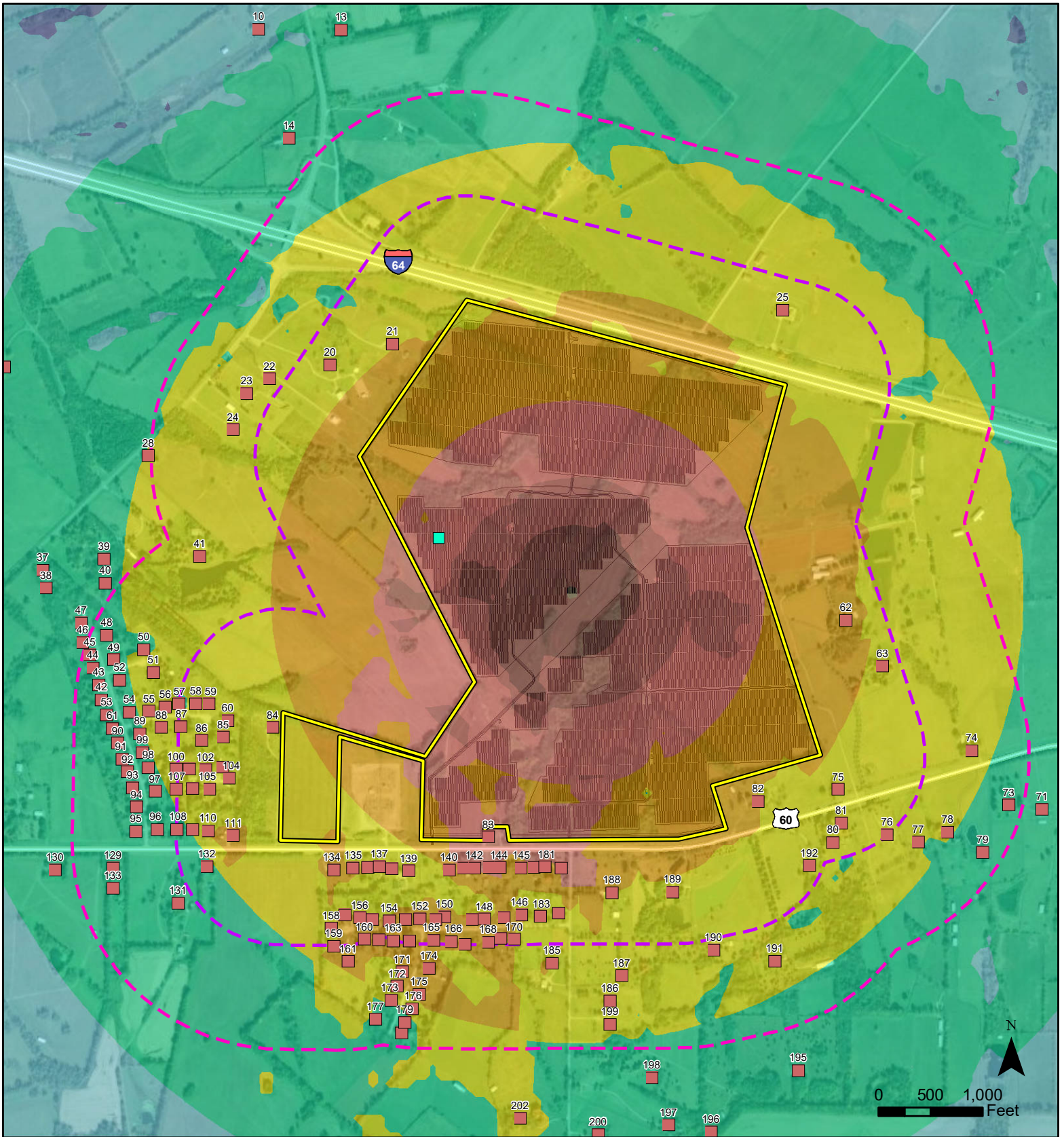
Figure 2 Received Sound Levels, Pile Driving Activities Bluegrass Plains Solar Project Fayette County, Kentucky
