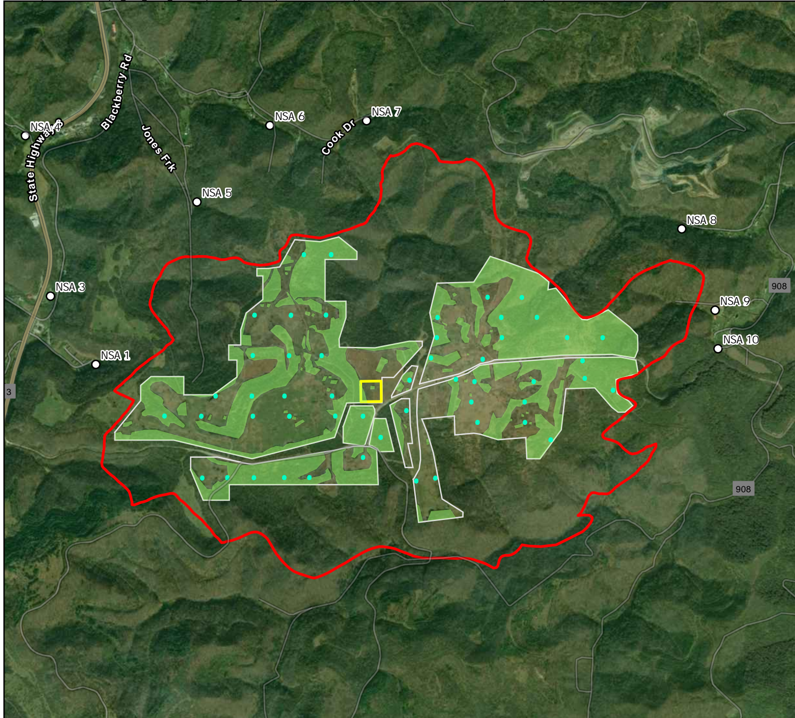
Figure 5 Tree Removal Map Lynn Bark Solar Project Lynn Bark Energy Center, LLC Martin County, Kentucky
