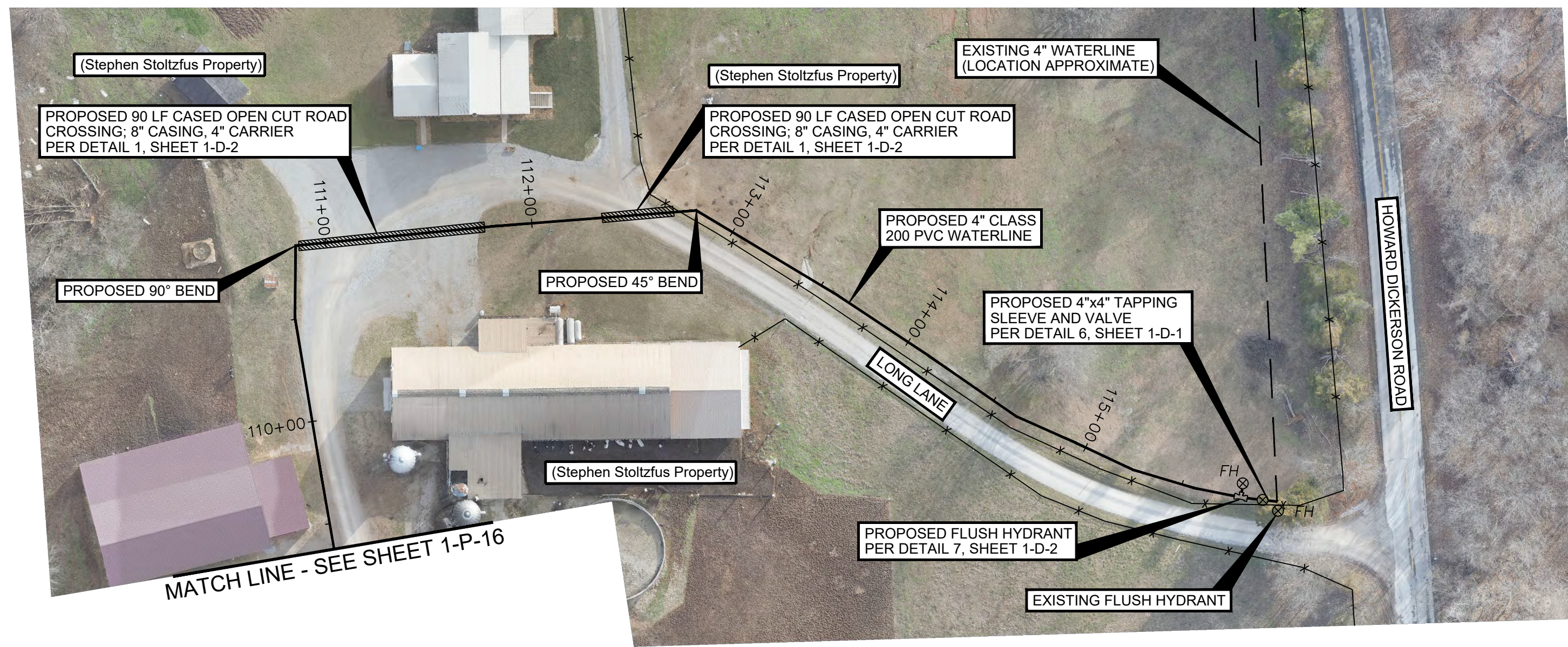
WATER LINE PLAN: STATION 109+40 TO 115+95
