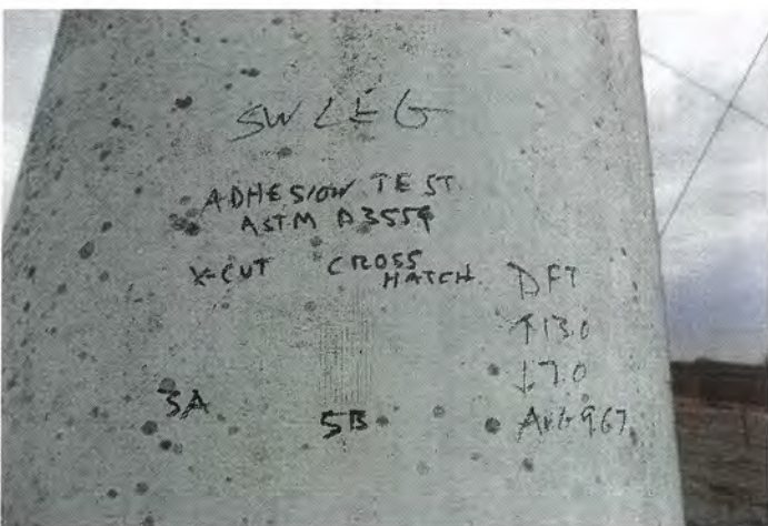
Photo shows the results of adhesion tests performed per ASTM D3359 on the southwest lower leg. The adhesion test results are a 3A and a 5B. The Dry Film Thickness (DFT) in the test area ranged from 7.0-13.0 mils and averaged 9.67 mils. The tank is a candidate for an overcoat.
