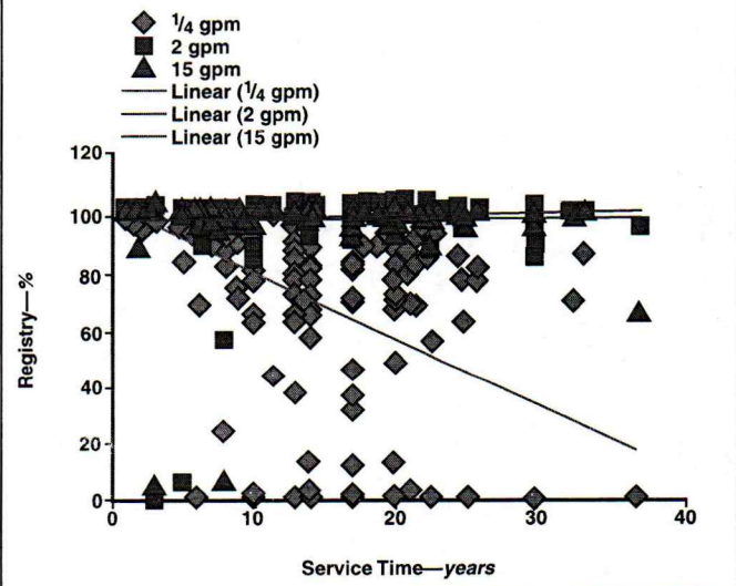
FIGURE 1 Service time versus registry 5/8- x 3/4-in. piston meters (Barfuss et al, 2011)
