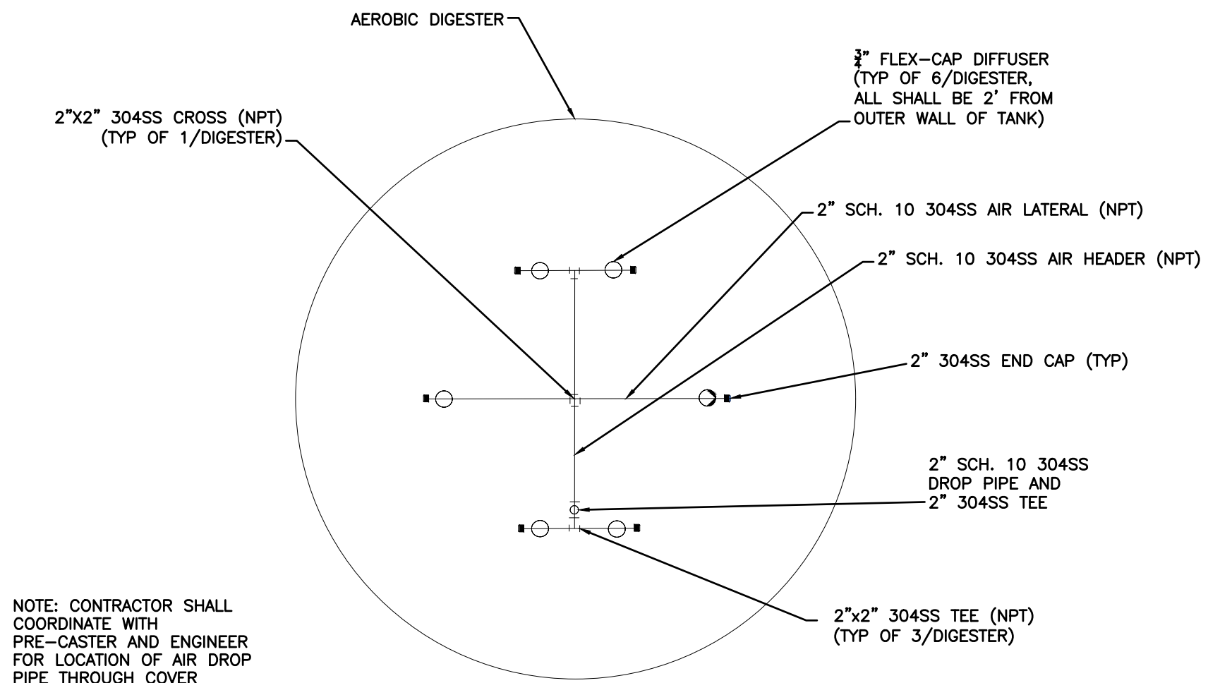
AEROBIC DIGESTER DIFFUSER LAYOUT PLAN NOT TO SCALE
