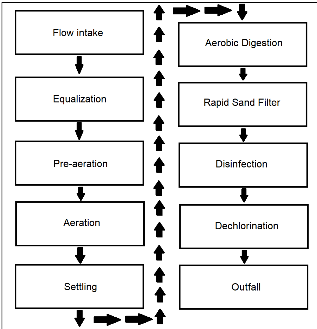
Facility Flow Diagram
