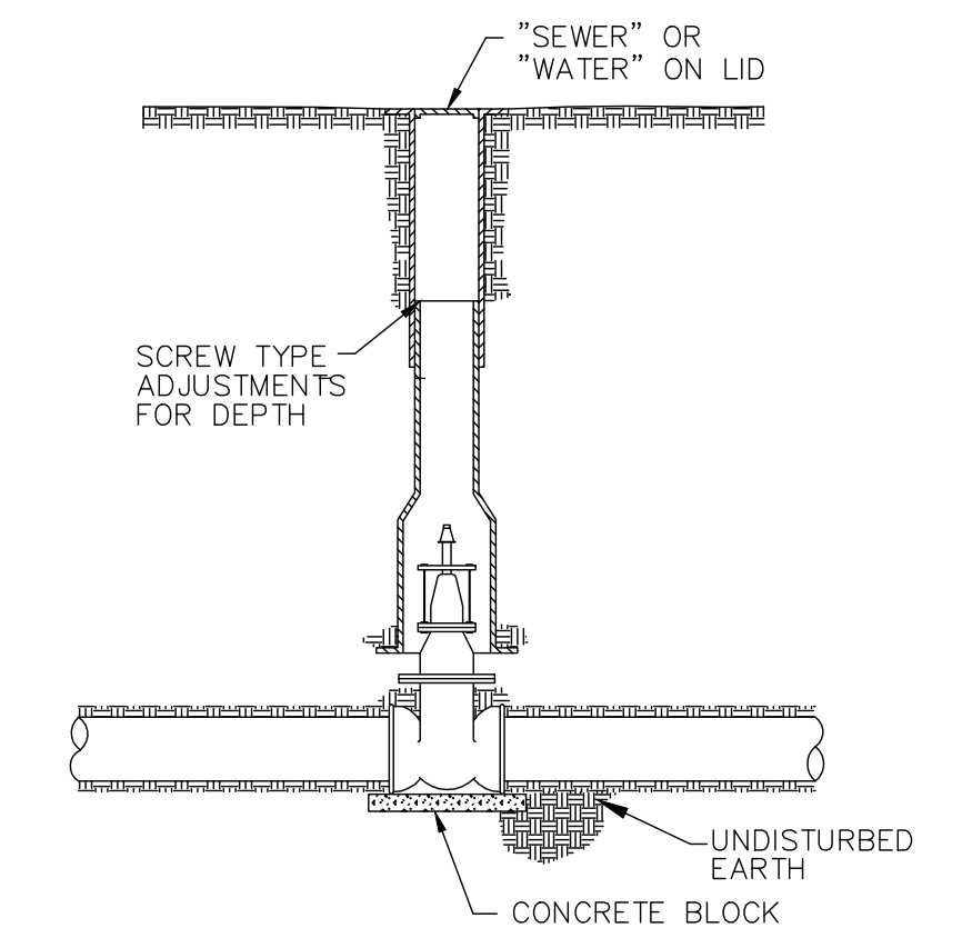
PIPE TO MANHOLE CONNECTION NOT TO SCALE
