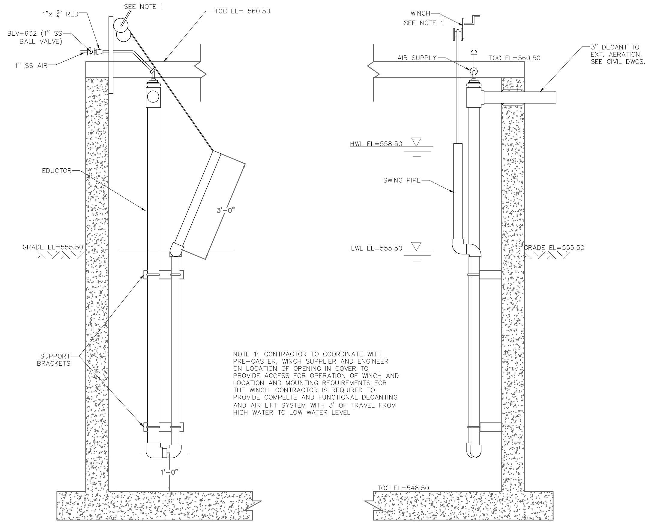
AIRLIFT PUMP SWING PIPE NOT TO SCALE
