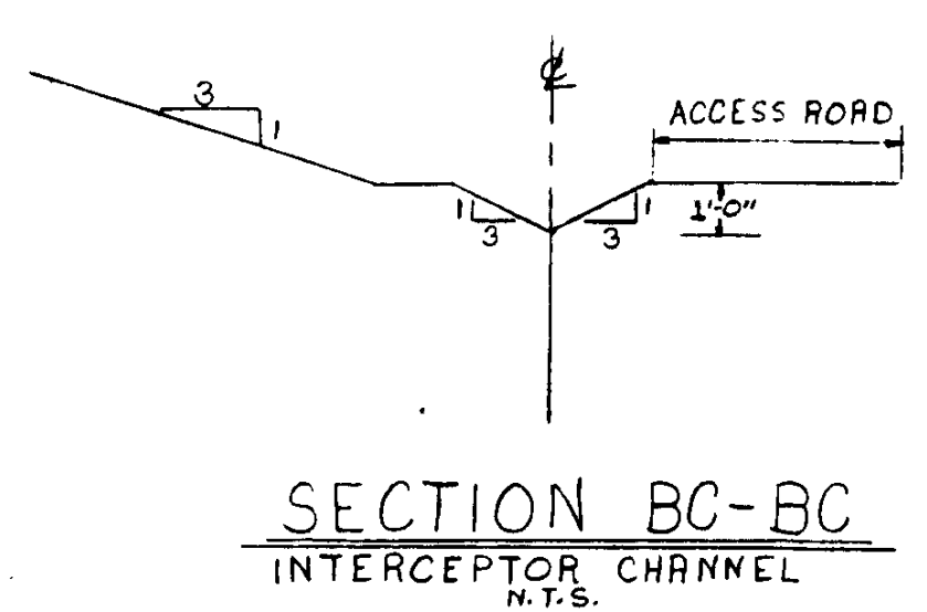
STATION 22+50
