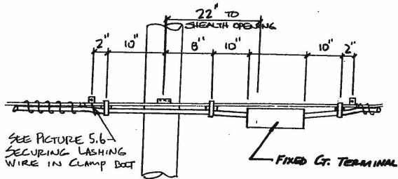
FIXED COUNT TERMINAL / SPICE THROUGH CABLE
