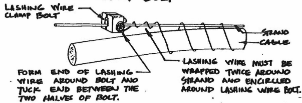
SECURING LASHING WIRE IN CLAMP BOLT
