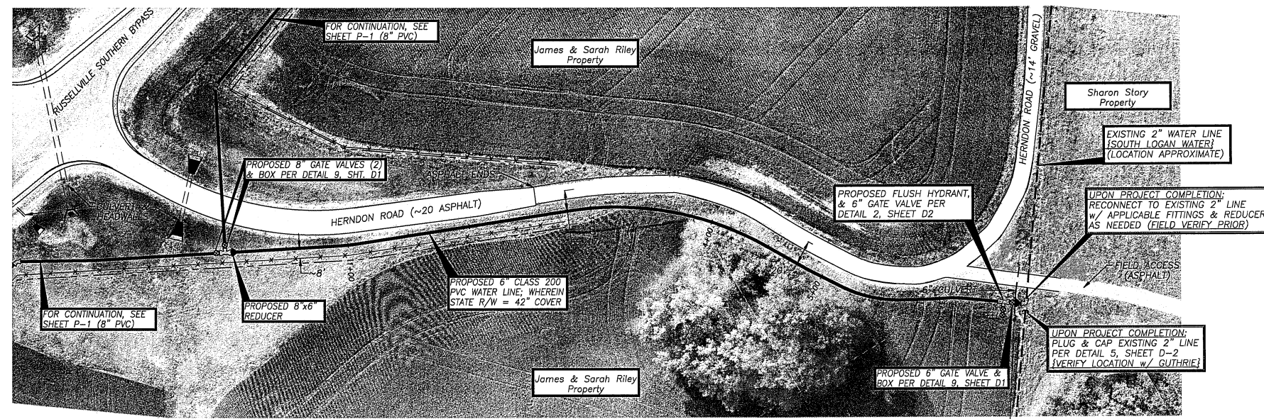
WATERLINE PLAN (HERNDON ROAD): STATION 0+00 TO 6+75
