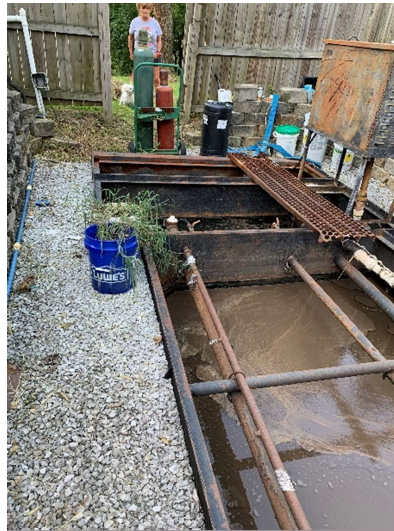
Aeration Tank, Clarifier, Contact Tank
