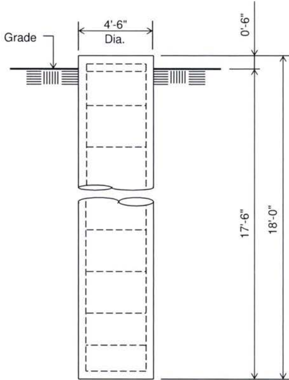
ELEVATION VIEW (10.6 cu. yds.) (3 REQUIRED; NOT TO SCALE)
