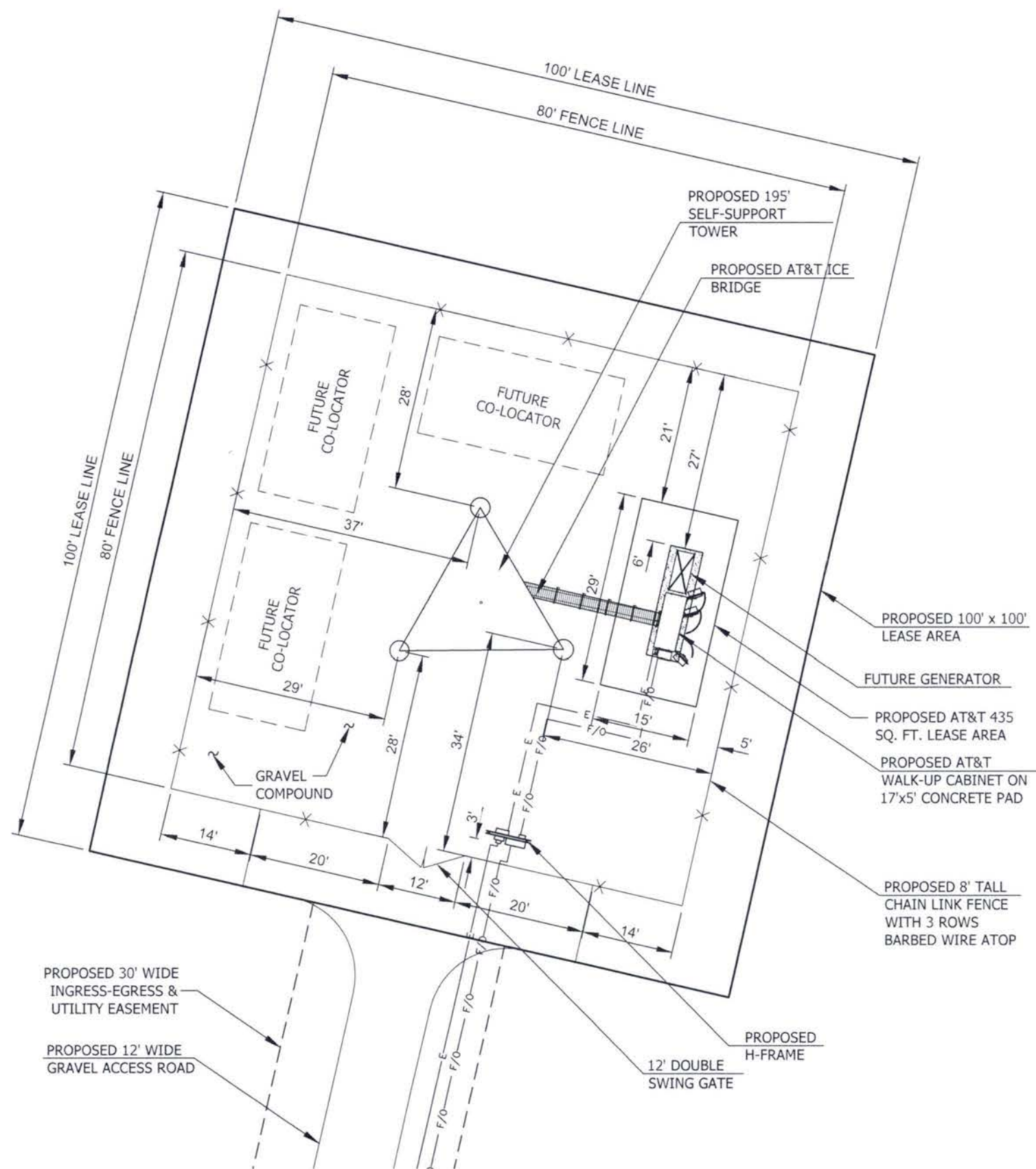
1 ENLARGED COMPOUND LAYOUT SCALE: 1"=20'
