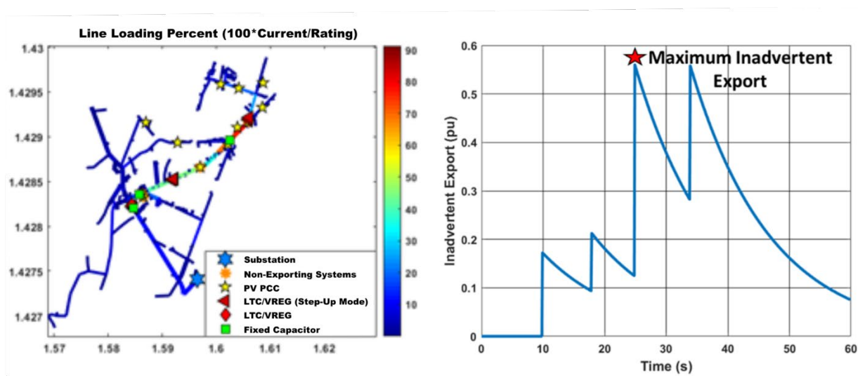
Figure XI. 20. Case 5 Rural Feeder: Line Loading at t=25s With 30s OLRT (Left) and Inadvertent Export Profile (Right)
