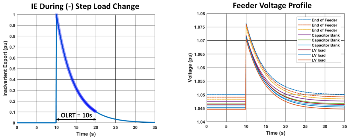
Figure 7. Case 6 Urban Feeder: Coincident Inadvertent Export Curve (Left) and Time Series RMS Maximum Voltage Profiles (Right)
