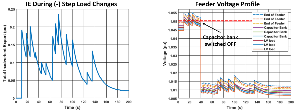
Figure XI. 13. Case 8 Urban Feeder: Non-Coincident Inadvertent Export Profile With 30s OLRT (Left) and Time Series RMS Maximum Voltage Profiles During the Same Time Period (Right)
