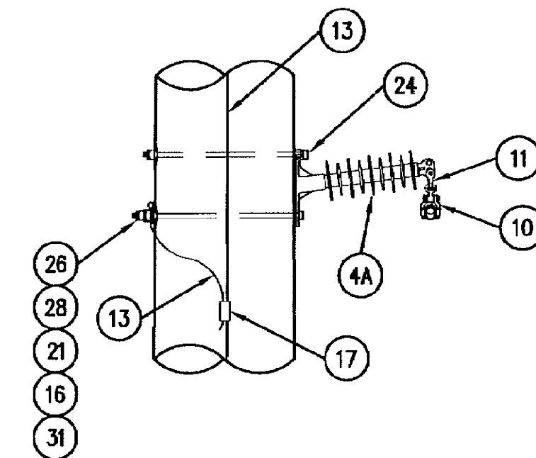
DETAIL 3 CONDUCTOR SUSPENSION ASSEMBLY
