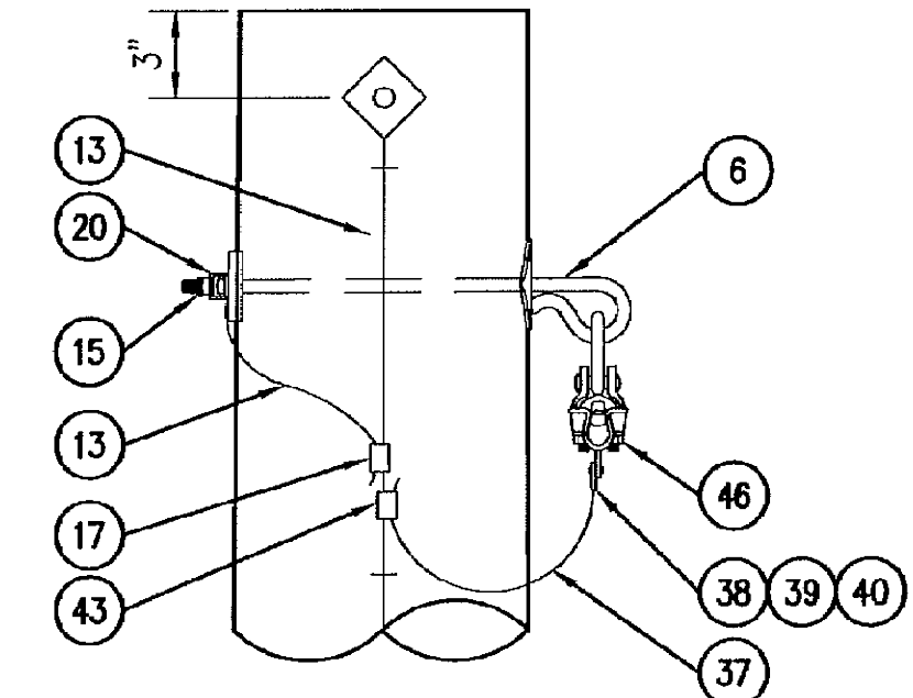
DETAIL 2 OPGW SUSPENSION ASSEMBLY
