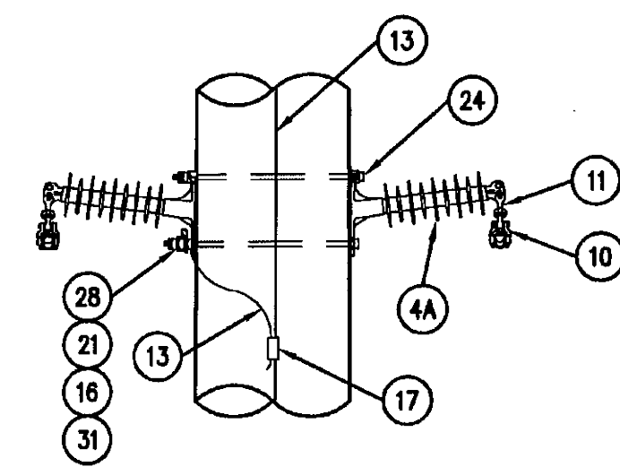
DETAIL 3A CONDUCTOR SUSPENSION ASSEMBLY
