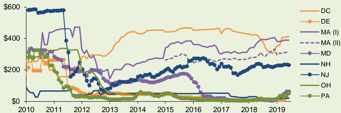
Average Monthly SREC Price (2018$/MWh)
