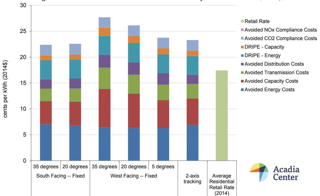
Figure 2: Grid Value of Solar PV in Massachusetts – 25-year Levelized Cost (2014$)
