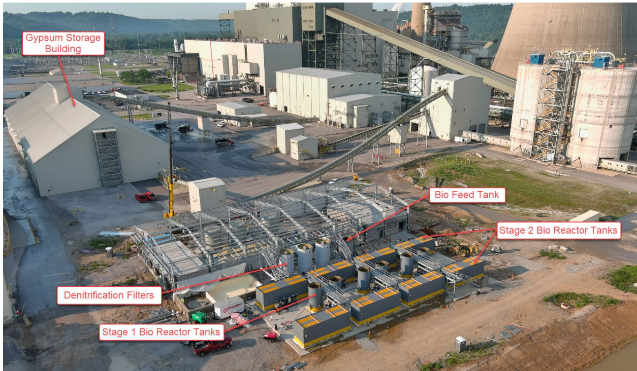
Trimble County – ELG Water Treatment Future Location – July 2022
