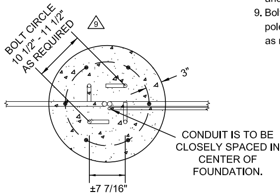
FOUNDATION DETAIL
