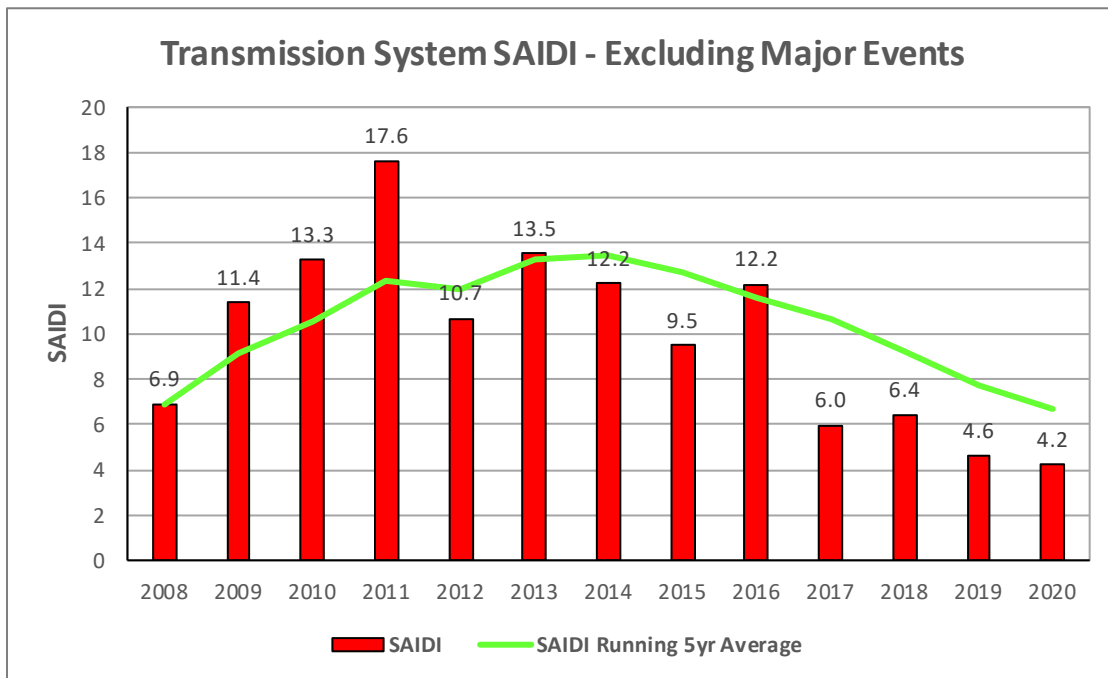
Figure 1: Combined Transmission SAIDI 2008-2020
