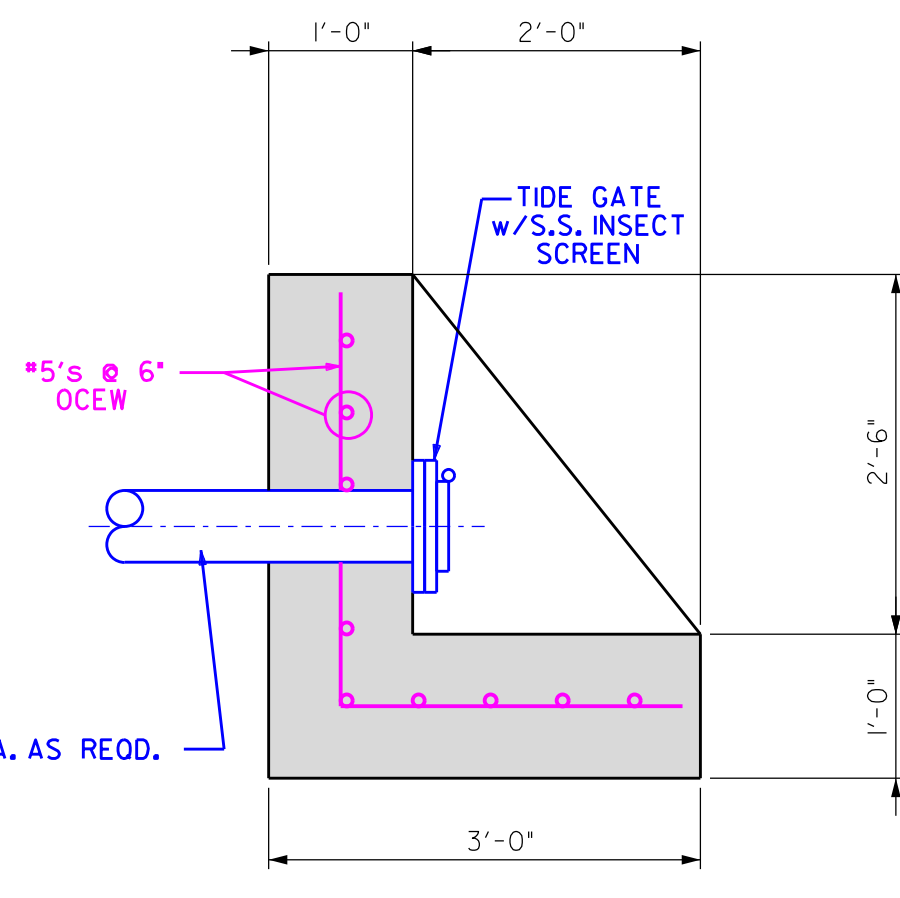
HEADWALL DETAIL NO SCALE
