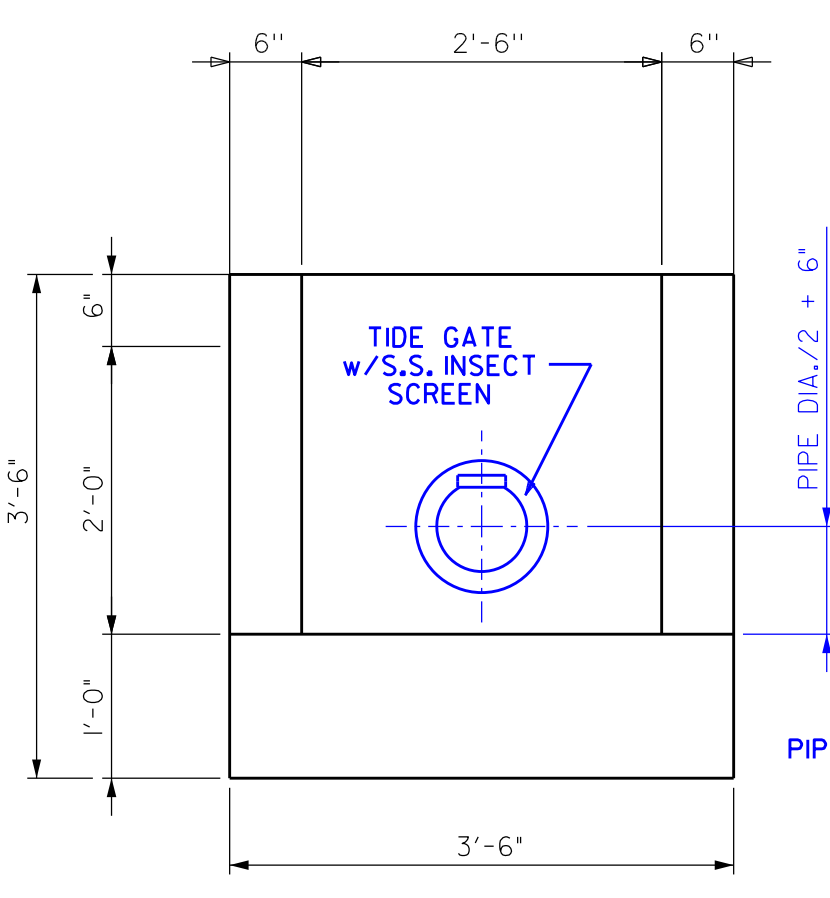
HEADWALL DETAIL NO SCALE
