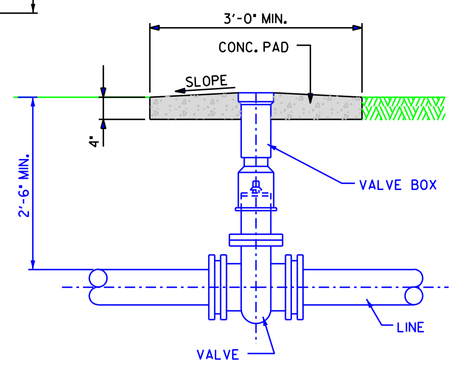
TYPICAL VALVE SETTING DETAIL NO SCALE
