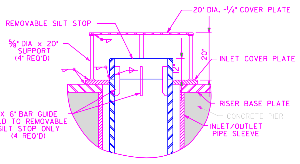
REMOVABLE SILT STOP - DETAIL NO SCALE
