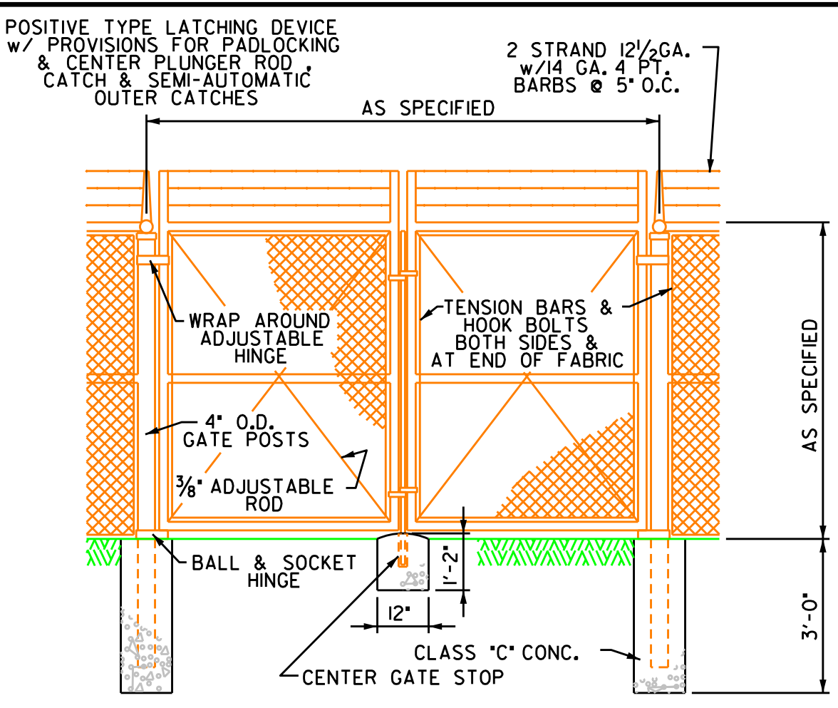
FENCE GATE DETAIL NO SCALE
