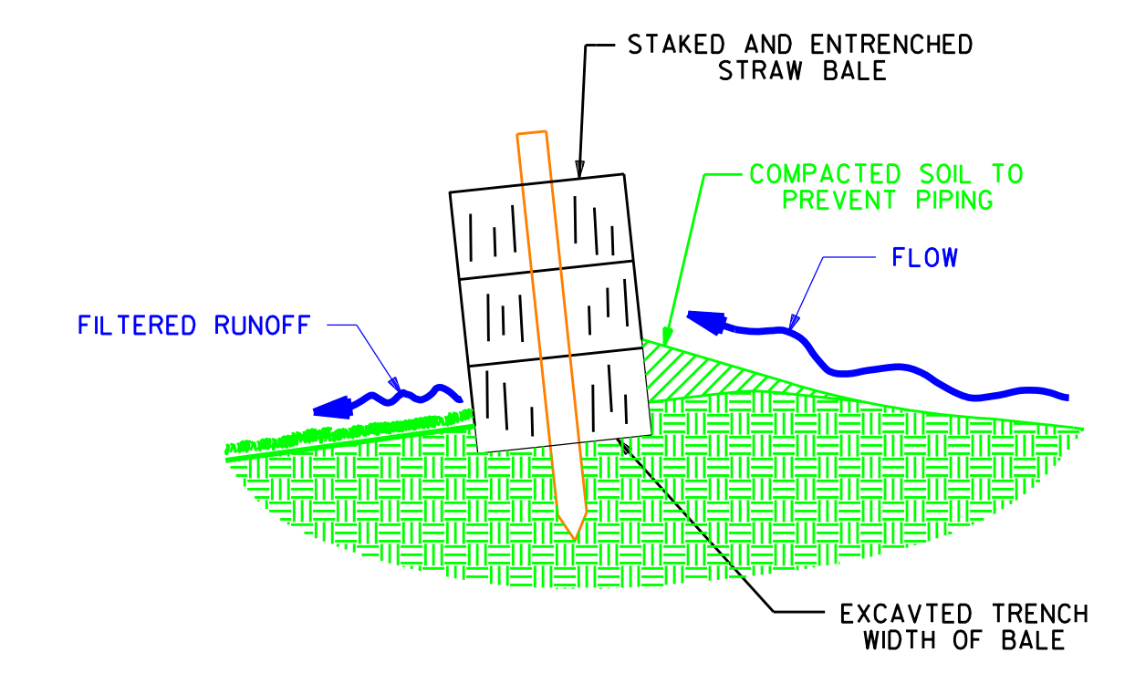
NOTE: WEDGE LOOSE STRAW BETWEEN BALES STRAW BALE BARRIER SCALE: 1/2" = 1'-0"
