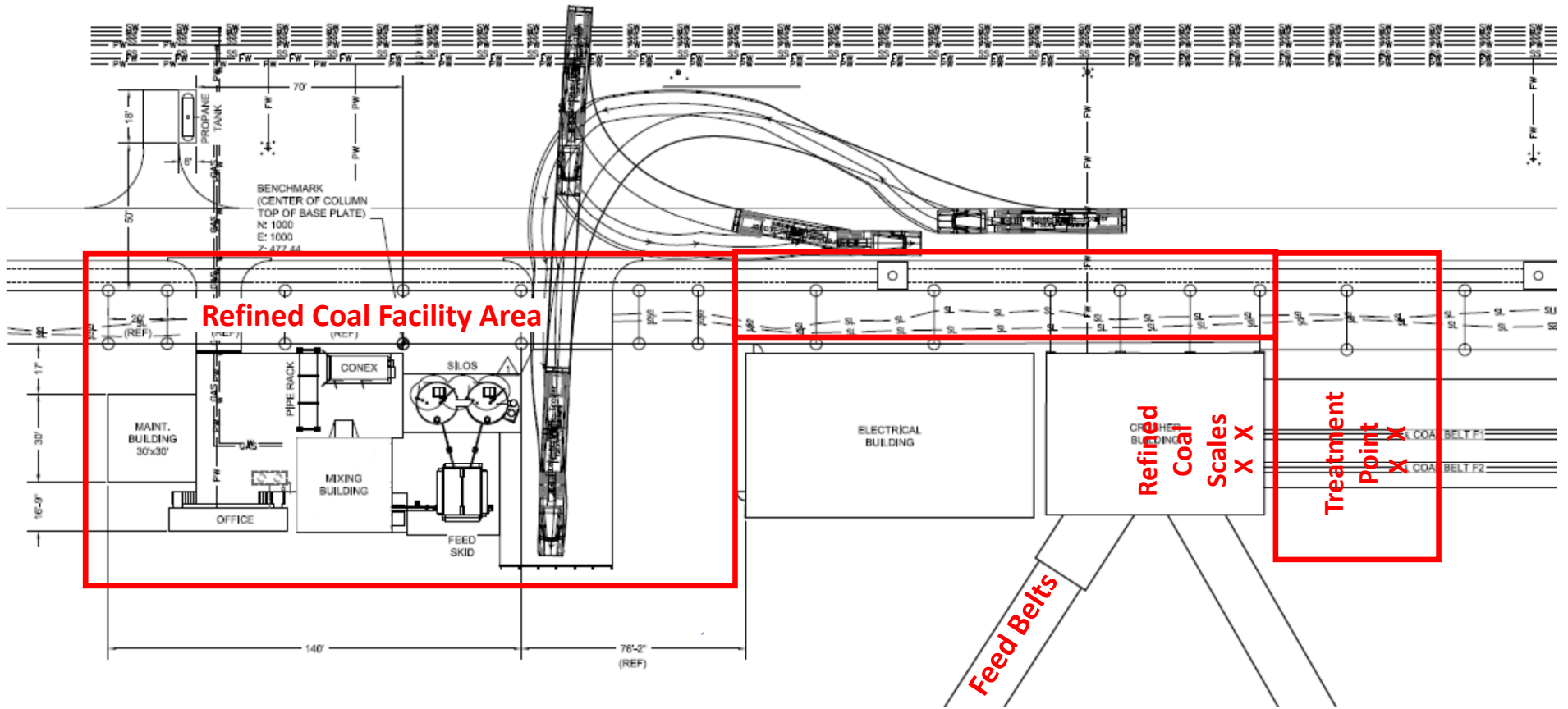
Trimble County Station Refined Coal Facility Map
