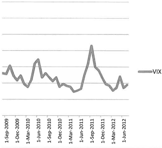
CHART 1 Monthly VIX
