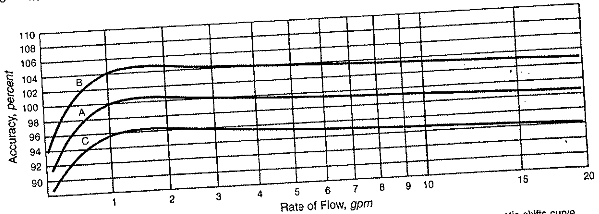
Figure 5-1 Effect of modifying change-gear combinations in typical \frac{5}{8} -in. (15-mm) meter
