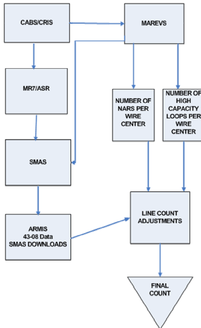
Retail & Resale Business Line Data Flow
