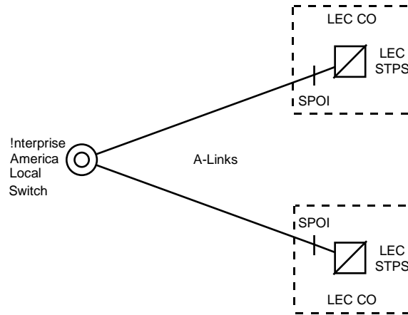
Figure 6. A-Link Interface
