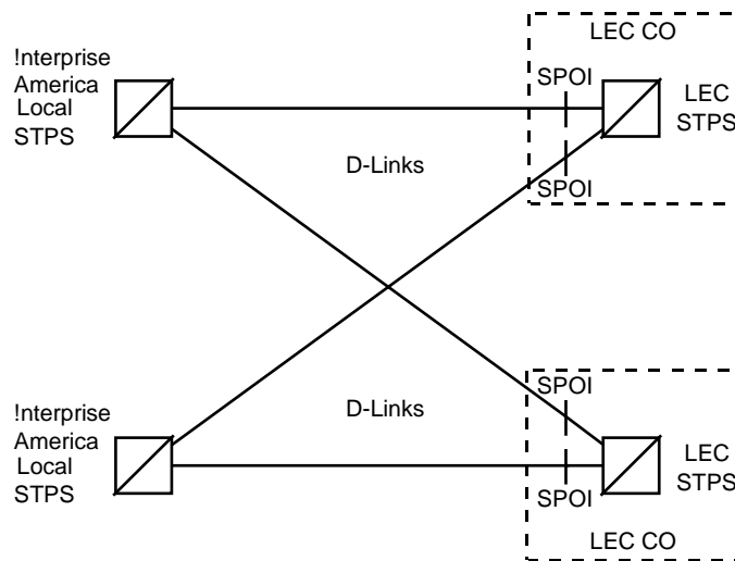
Figure 7. D-Link Interface
