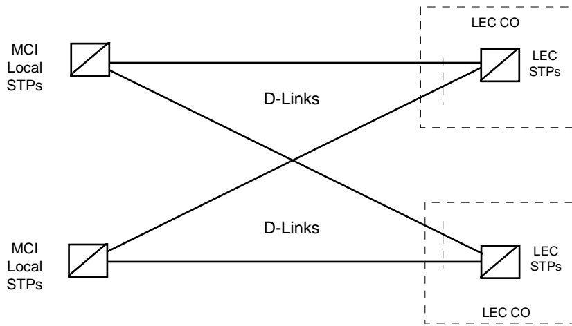
FIGURE 10. D-LINK Interface
