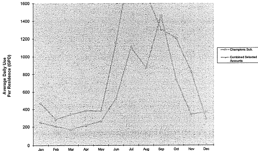
Graph - 26 Champions Subdivision Average Daily Usage With Combined Selected Accounts 2005
