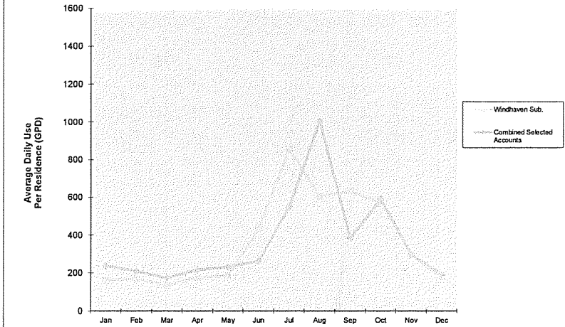
Graph - 34 Windhaven Subdivision Average Daily Usage With Combined Selected Accounts 2005
