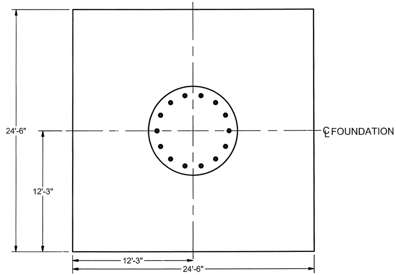
PLAN VIEW (REINFORCEMENT NOT SHOWN FOR CLARITY)
