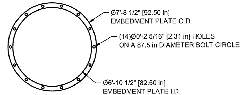
EMBEDMENT PLATE DETAIL
