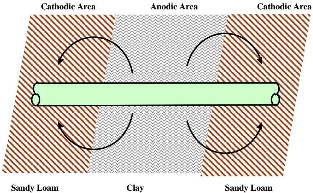
Figure III-18 Galvanic Corrosion
