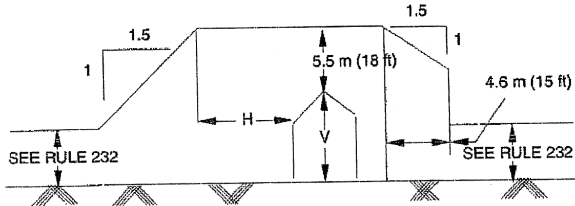
Fig 234-4(b): Clearance Envelope for Grain Bins Filled by Portable Augers, Conveyors, or Elevators
